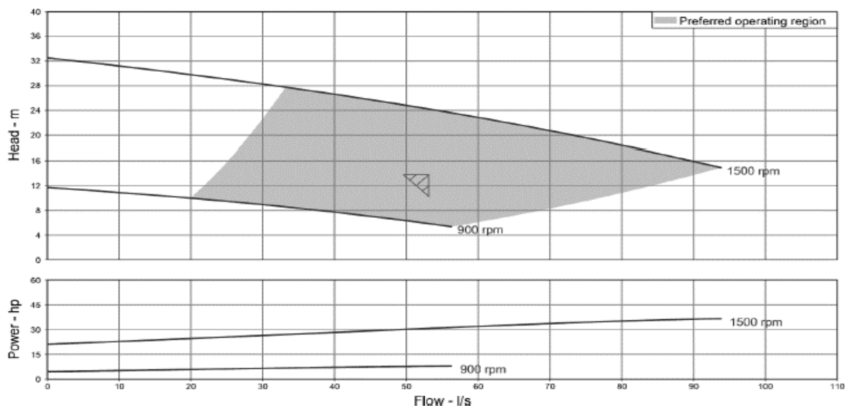
CURVA DE PERFORMANCE MOTOBOMBA
